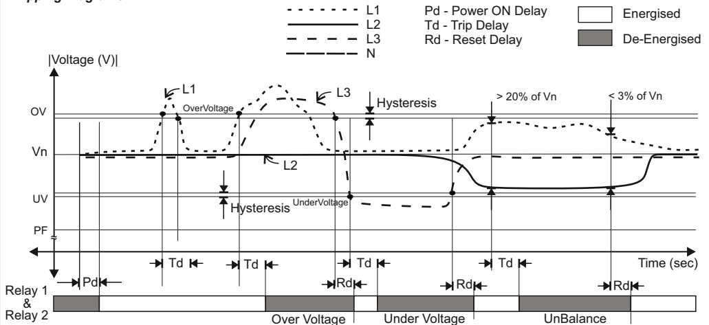
Figure 1 : OV, UV & UB Tripping functionality for 3 Phase System with default Energised Relay
