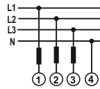
3Phase 4Wire
